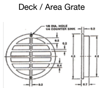
Round Grate
